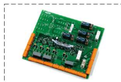
KM50006052G01 Kone ADO board
